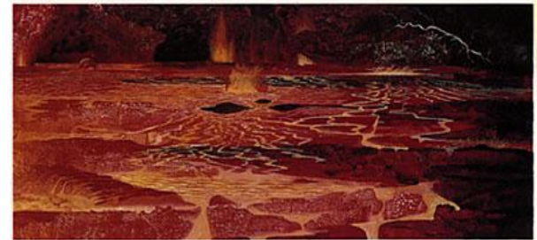
44 Semi-molten surface of the Earth 4500 million years ago
