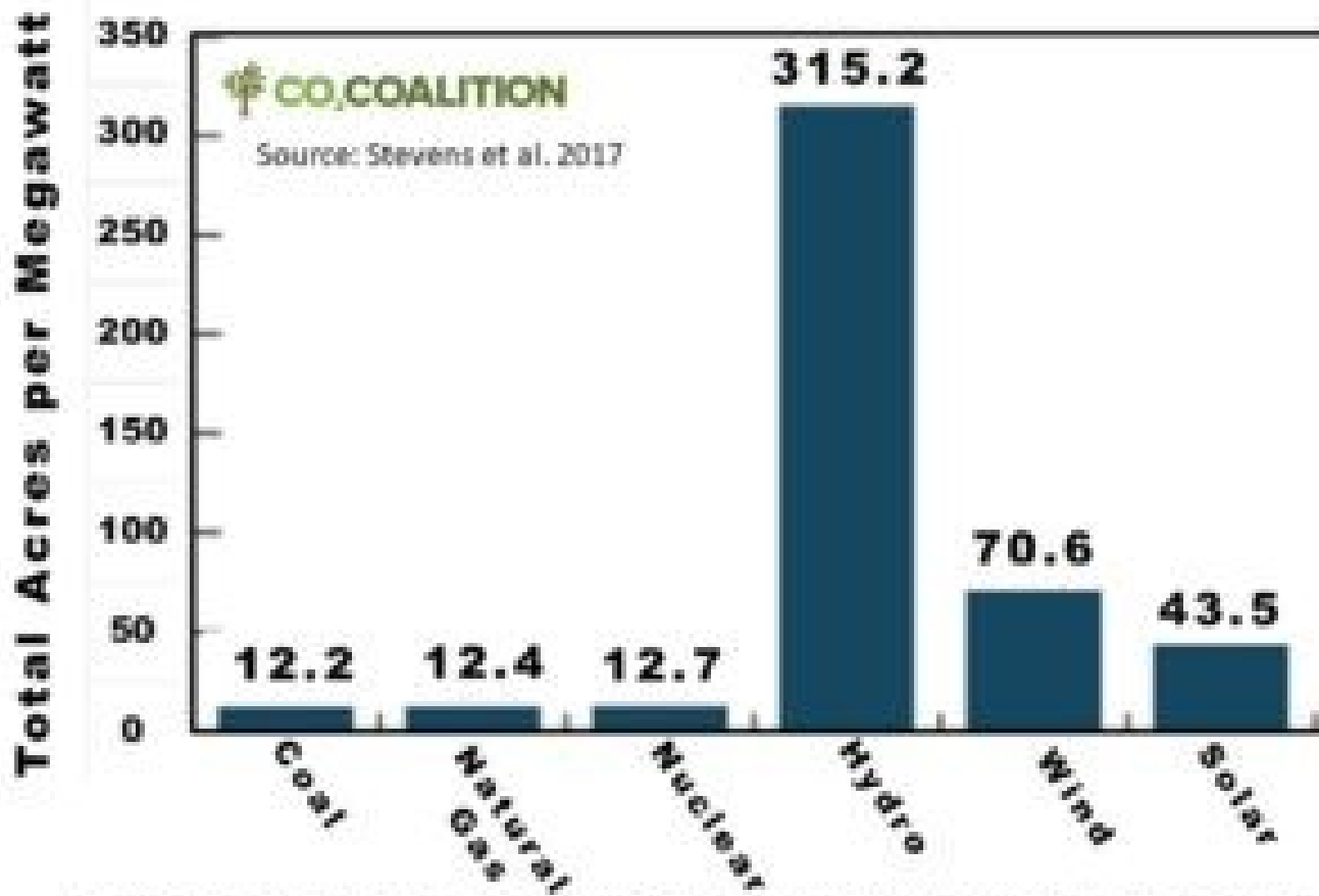
Physical footprint per megawatt of energy produced using various energy technologies
