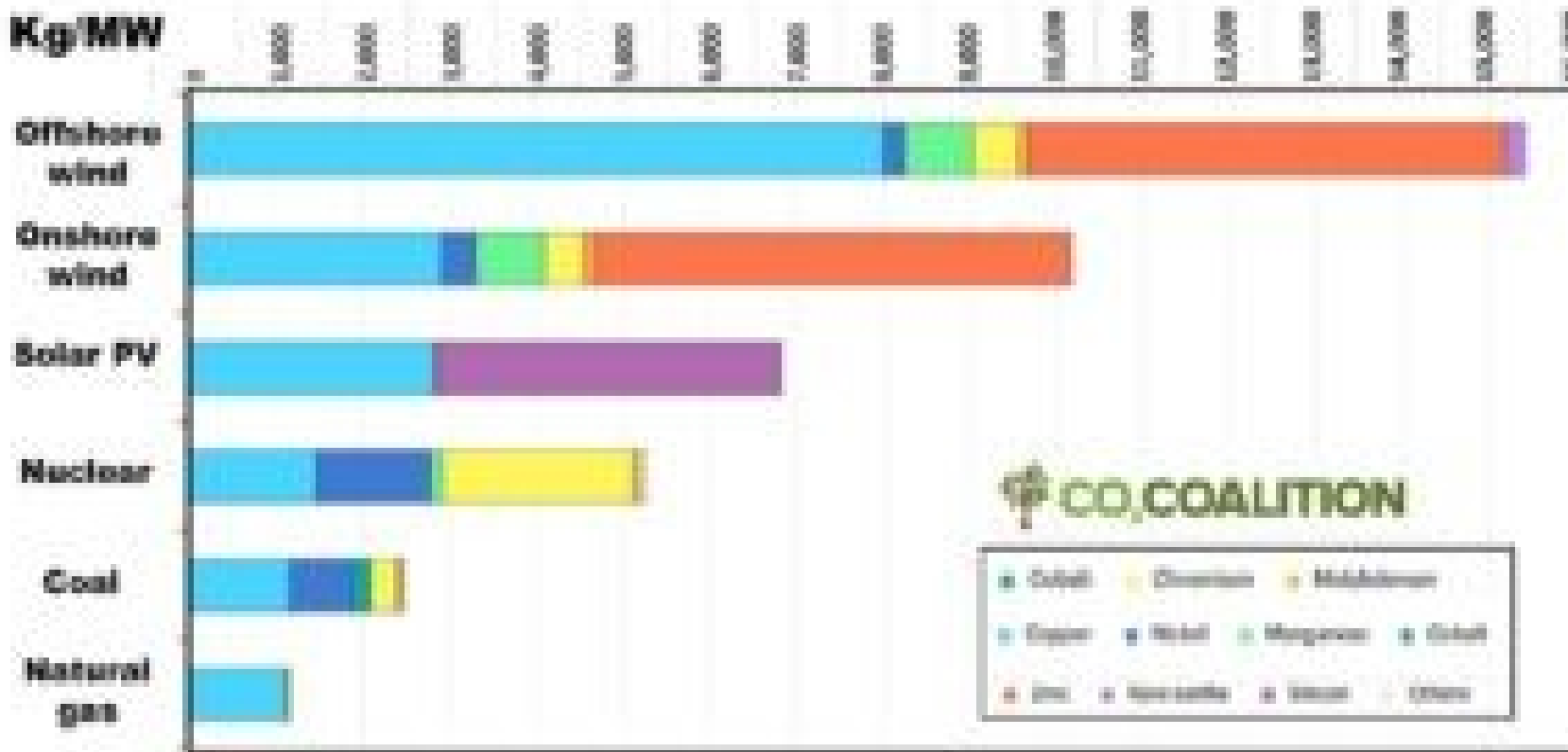
Metals demand for clean energy technologies compared to other power generation sources
