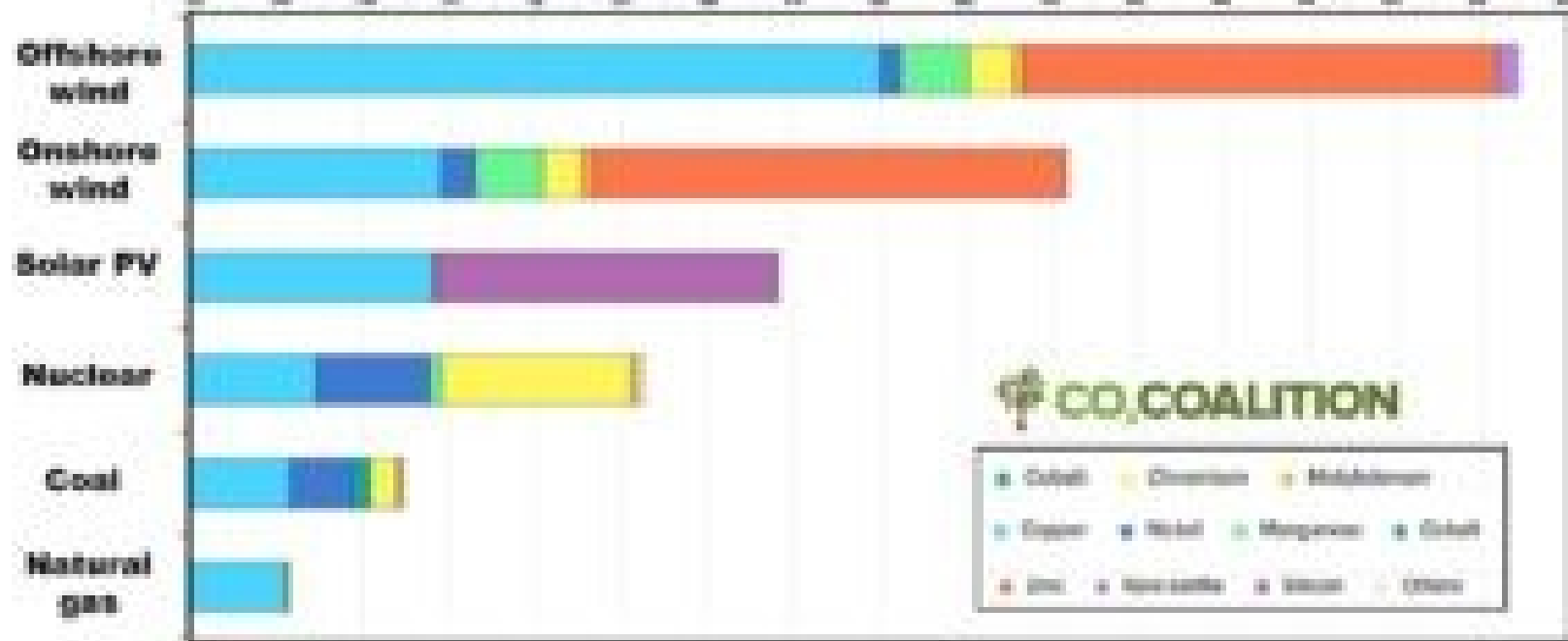
Metals demand for clean energy technologies compared to other power generation sources
